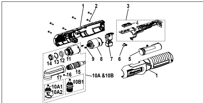
Figure 6: Exploded View CTNN2040/CTNNQ2040
