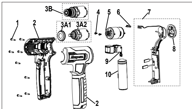
Figure 6: Exploded View CTNN3040/CTNNQ3040
